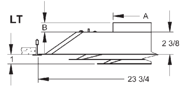
1200, ROUND NECK 2-CONE LOUVERED FACE DIFFUSER, LAY-IN
